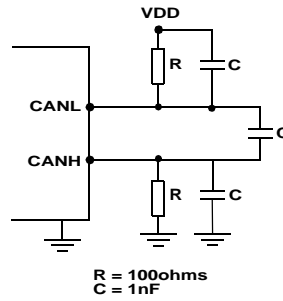
Figure 4. Test Circuit for AC Characteristics
